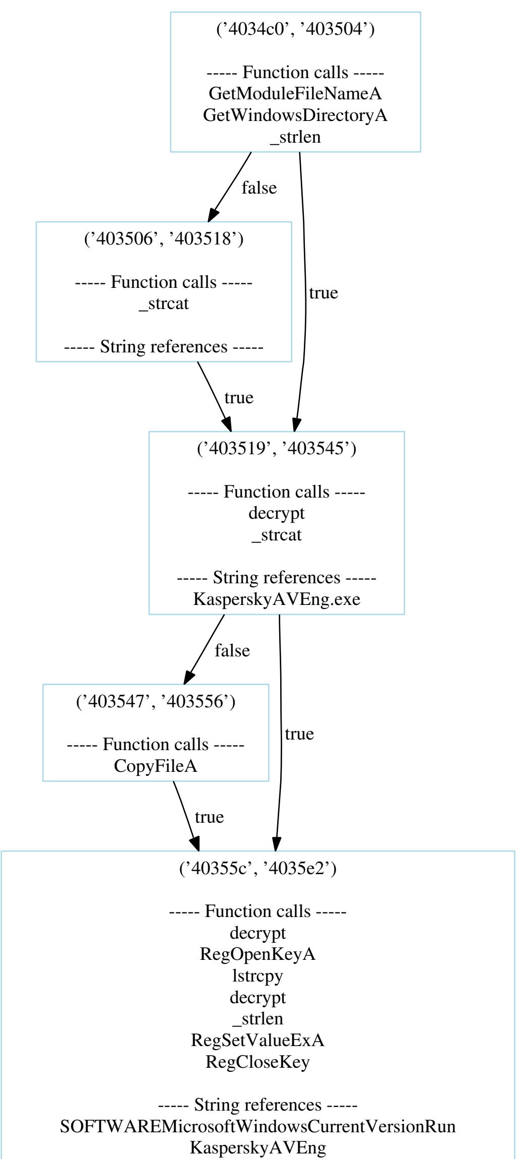
Control Flow Graph for NetSky.V Install function
